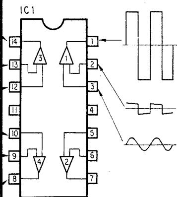
WAVE FORMS OF IC1 —
